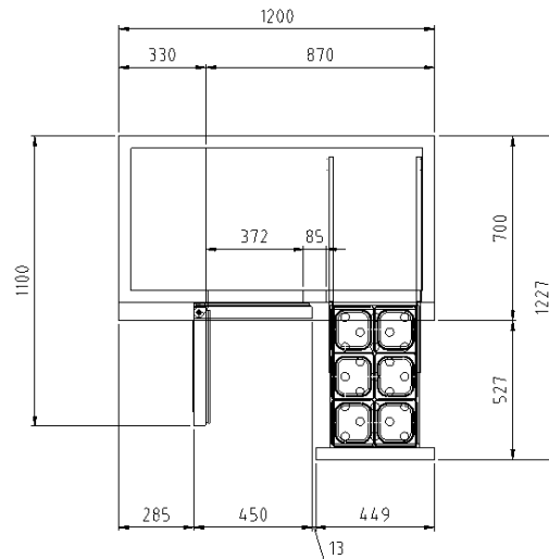
PLAN VIEW
