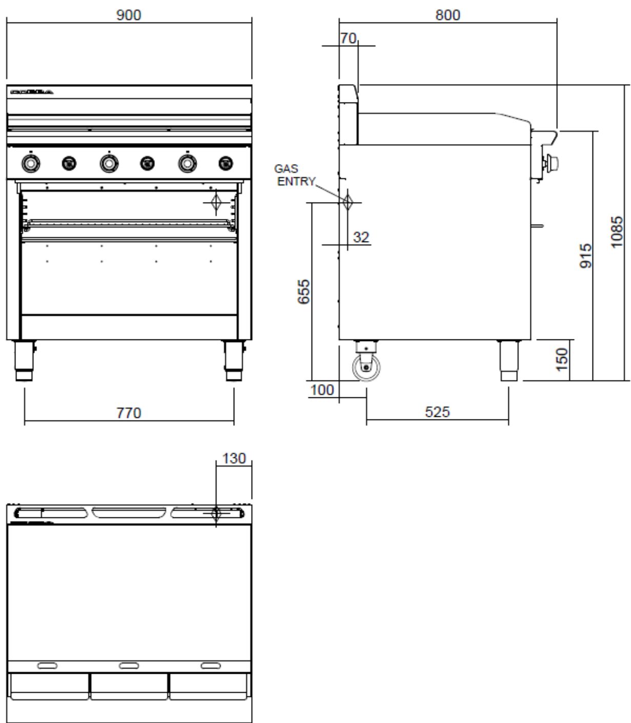
CT9 Gas Griddle Toaster (900mm)
