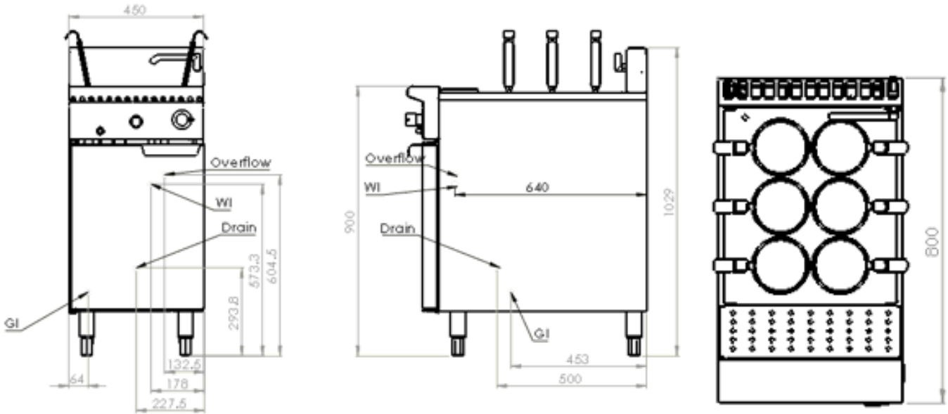
Figure 1: Plumbing Connections -Verro NC-6 (800 deep)
