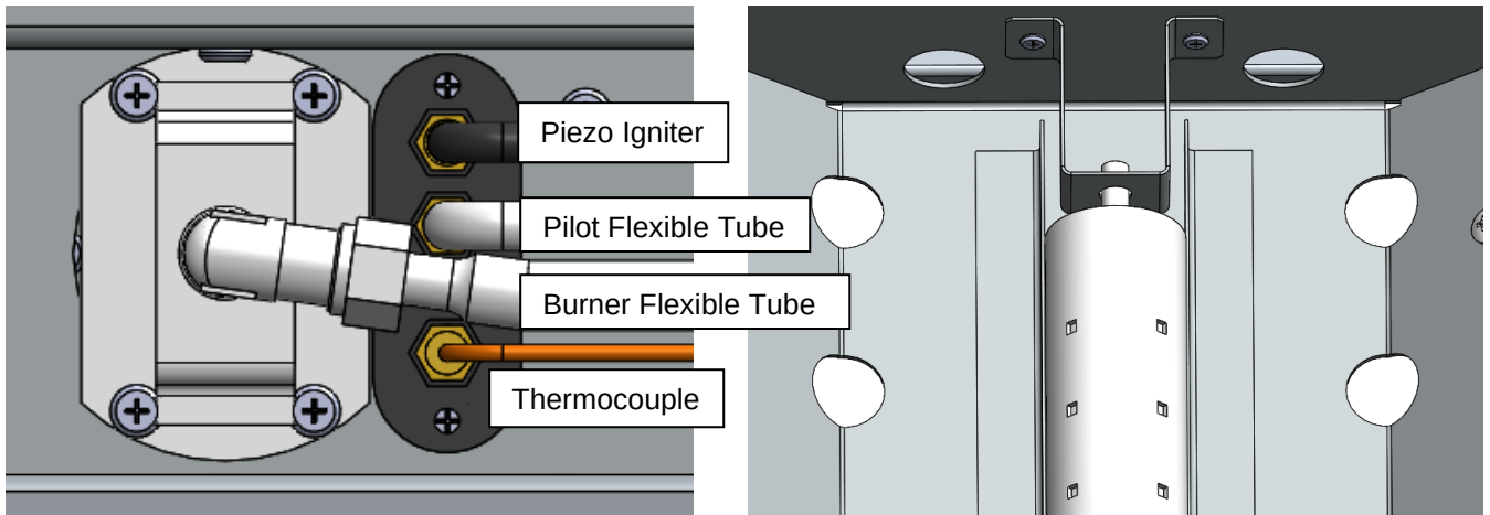
Figure 19: Oven Series Internal Components
