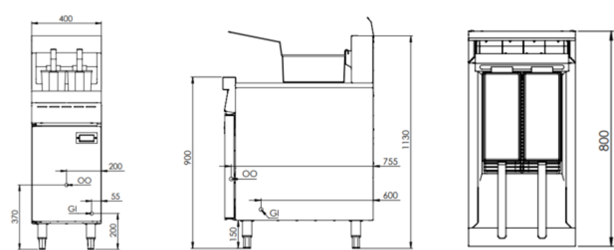
FIGURE 4: Plumbing Connections: RF-400
