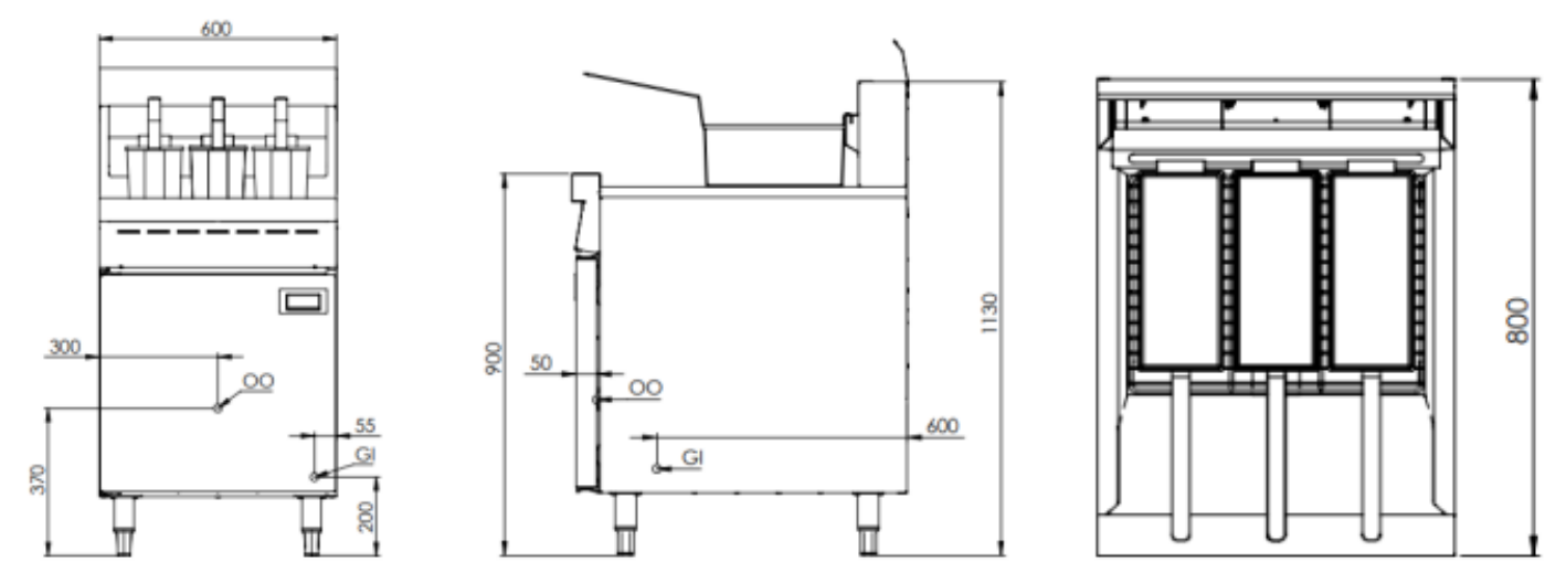
FIGURE 5: Plumbing Connections: RF-600
