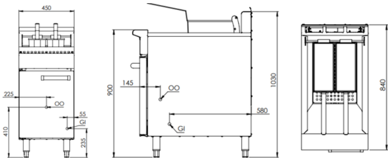
FIGURE 2: Plumbing Connections: Verro TF-451/Black TF 451
