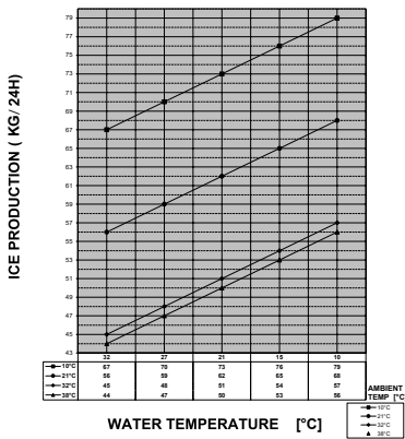
ICE PRODUCTION DIAGRAM
