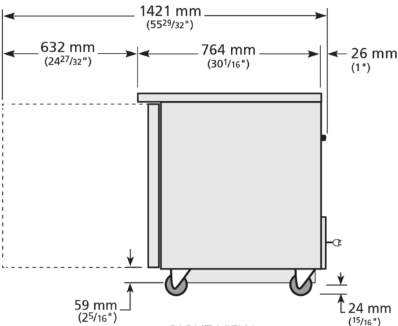
RIGHT VIEW
