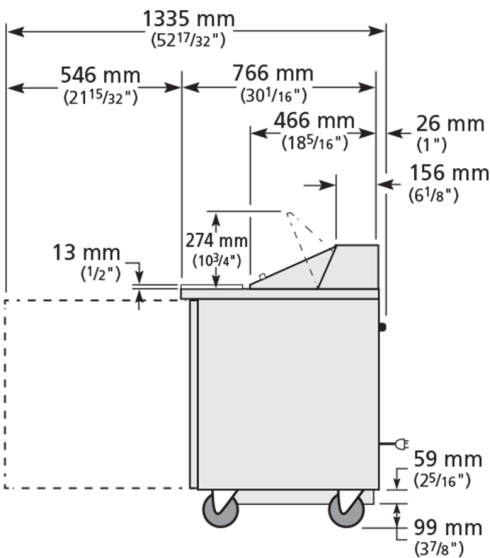
RIGHT VIEW
