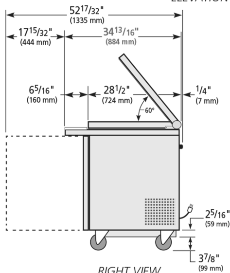
RIGHT VIEW
