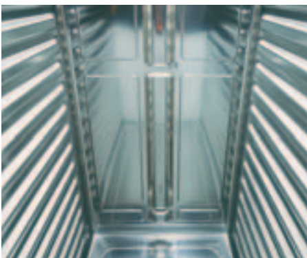
Easy to keep hygienic: Tightly welded interior with deep-drawn support rails and rounded corners (corresponds to hygiene version H3).
