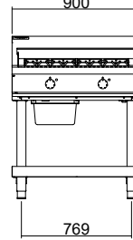
CHLB8900EDE-LS
