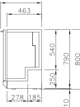
SIDE VIEW (800mm)
