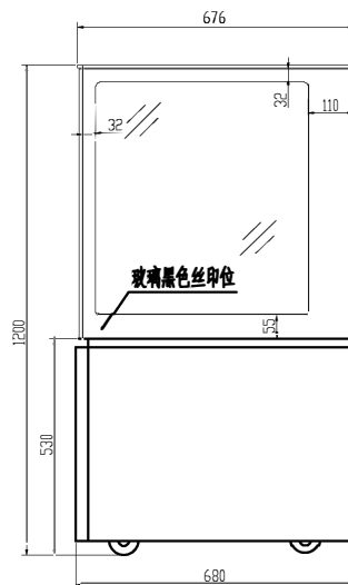
SIDE VIEW 左侧视图
