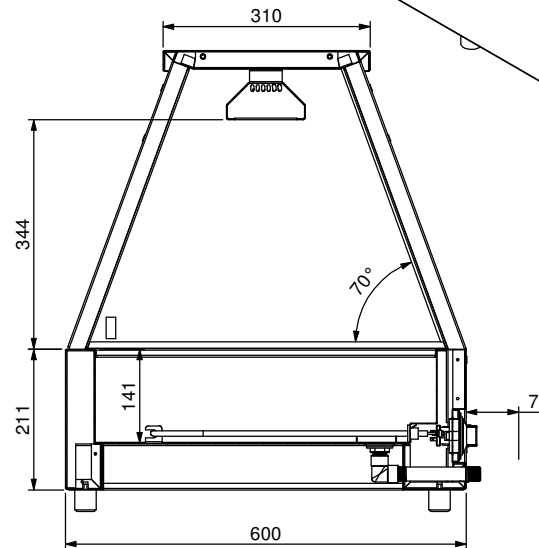
SECTION BH-BH
